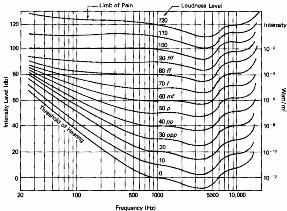
Figure 1-4 Fletcher-Munson curves of equal loudness level (isophons).
