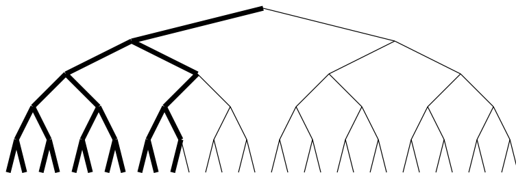
Figure 12.9: Bounded-backtrack search
