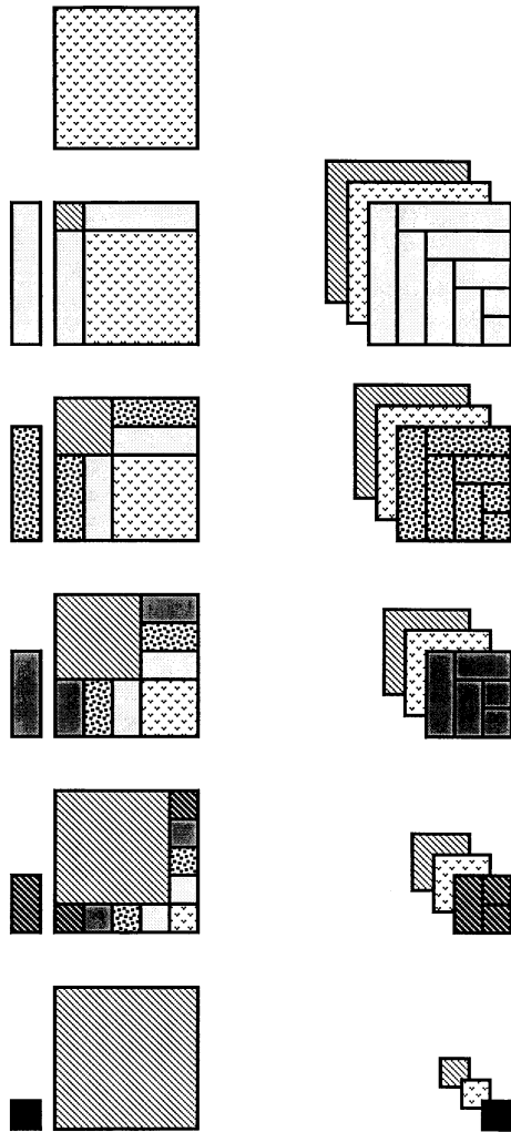
Figure 1: Sum of squares
