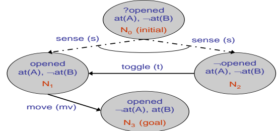
Figure 1: A contingent solution in AND/OR forward search
