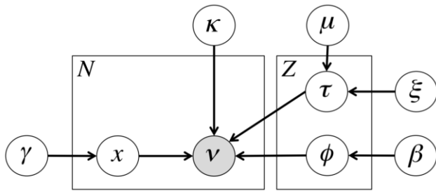
Probabilistic Topic Models
