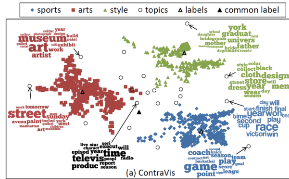
Visual Comparative Text Mining
